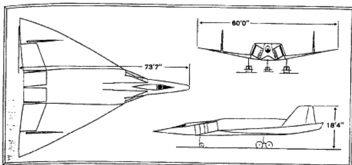
Convair KINGFISH
