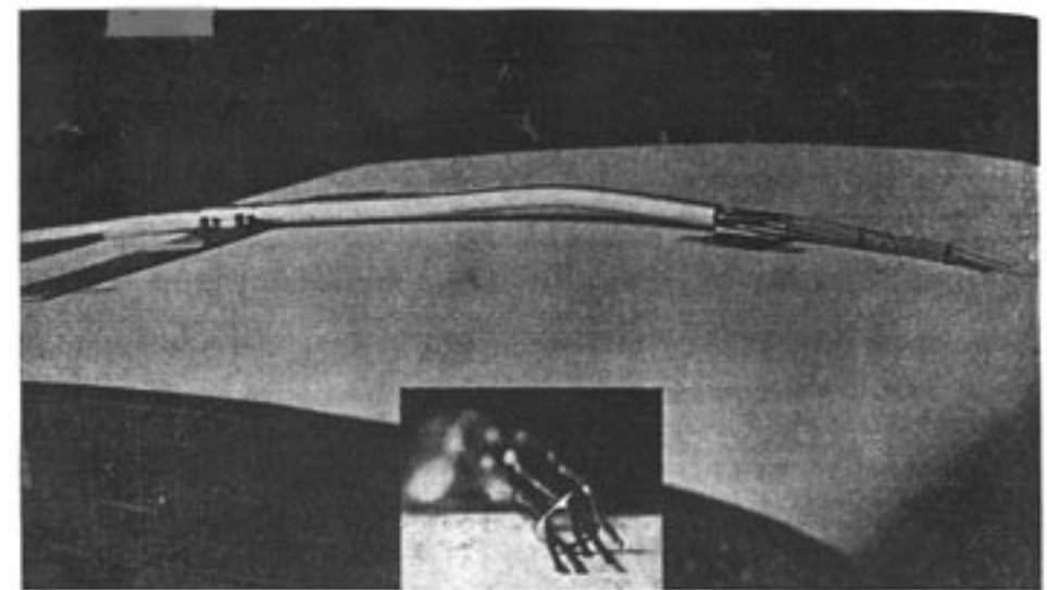
Fig. 3. Photographs of the five-tube head used for exploring the transition region in flight. The four tubes with orifices in the form of horizontal slits register total pressure at various distances from the wing surface, their outside dimensions at the front end are 0.012 in. deep and 0.064 in. wide. The tube with round closed end registers static-pressure.
