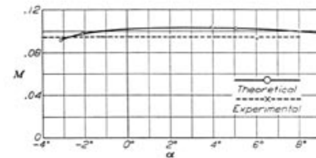
FIGURE 4.—Moment against angle of attack
