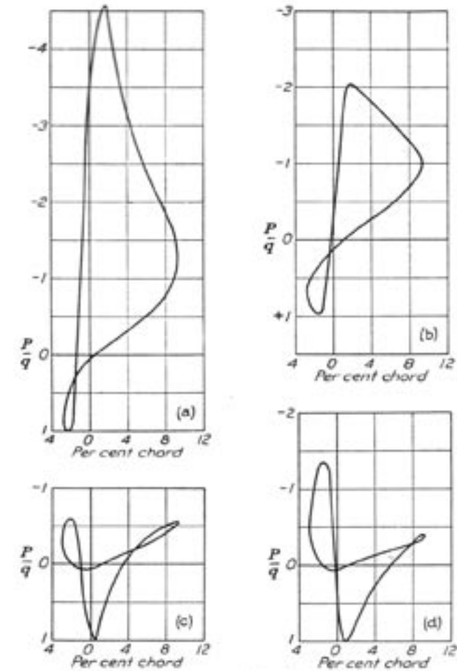
FIGURE 3.—Theoretical pressure distribution along y-axis of Clark Y (a) \alpha = 0^\circ , (b) \alpha = 2^\circ , (c) \alpha = -1^\circ , (d) \alpha = -3^\circ
