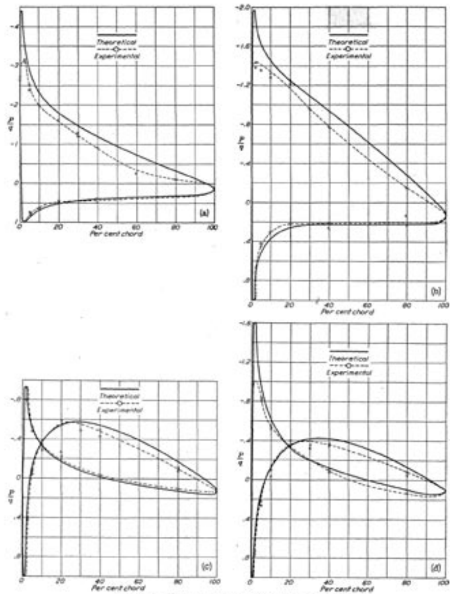
FIGURE 3.—Pressure-distribution curves along x-axis of Clark Y, C_{L_{max}} = 1.6 at \alpha = 0^\circ . (a) \alpha = 0^\circ , (b) \alpha = 2^\circ , (c) \alpha = -1^\circ , (d) \alpha = -3^\circ
