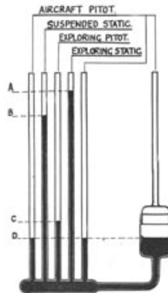
Fig. 4. Diagram illustrating manometer connection. The "impact pressure" of the aeroplane's air-speed is indicated by the distance BD, the total-pressure loss at the exploring pitot tube by the distance CD and the pressure (below atmospheric) at the exploring static-pressure tube by the distance AB. When the total-pressure loss and static-pressure are expressed in sufficient form by dividing by the impact pressure the values obtained are obviously independent of aeroplane lift or acceleration and of air or liquid density. The liquid generally used in the tubes is alcohol, but there are various heavy liquids of specific gravity up to 2.5 which can be conveniently used when the flight speed is very high.
