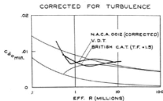
Fig. 10 - N.A.C.A. 0012 Airfoil Minimum Drag As Found from Different Tunnels
