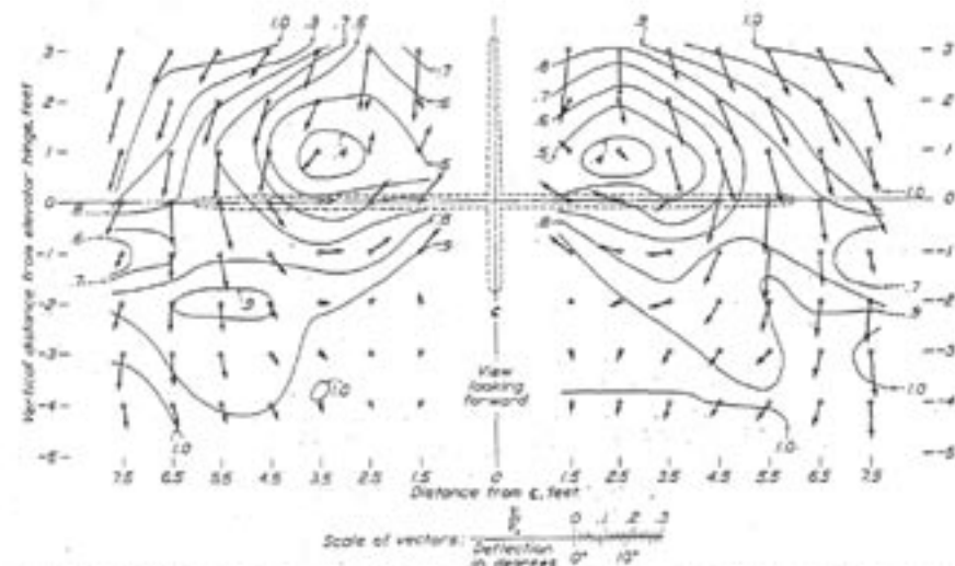
FIGURE 28.—Air flow at tail of McDonnell airplane in original condition, power off. Survey in vertical plane through stabilizer hinge line. The contours show the lines of the dynamic pressure behind the airplane in the dynamic pressure in the free air stream. The vectors show the components of the velocity in the plane of the survey. Angle of attack (thrust axis) = 14.7^\circ (corrected for tunnel effects). Lift coefficient = 0.84 .
