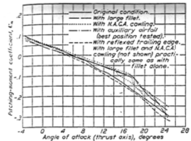
FIGURE 22.—Pitching moments of McDonnell airplane with various devices. Corrected for tunnel effects. Power off. Stabilizer 0.6° to thrust axis. Elevator 0° to stabilizer.
