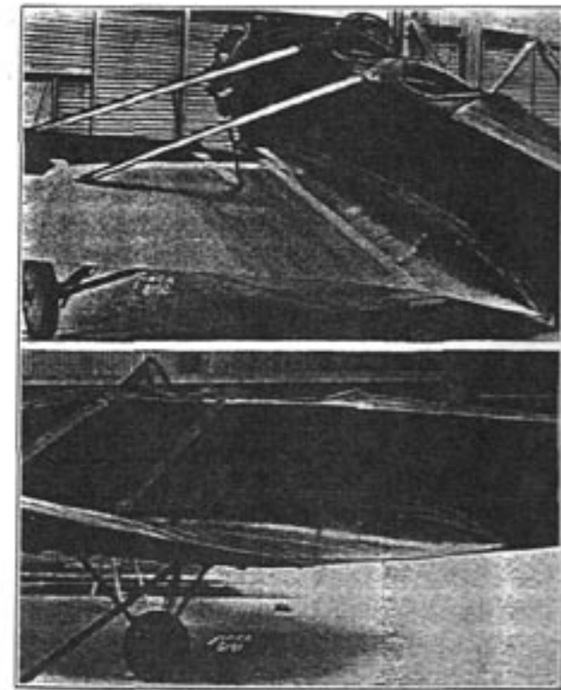
FIGURE 11.—Reflected trailing edge with fillet on 36-foot winged airplane.
