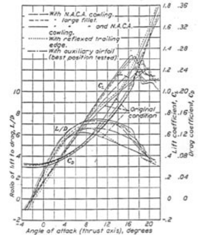
FIGURE 18.—Lift and drag of McDonnell airplane comparing various devices. Corrected for tunnel effects. Power off.
