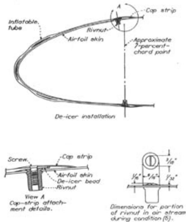
Figure 2. Rubber inflatable deicer details.
