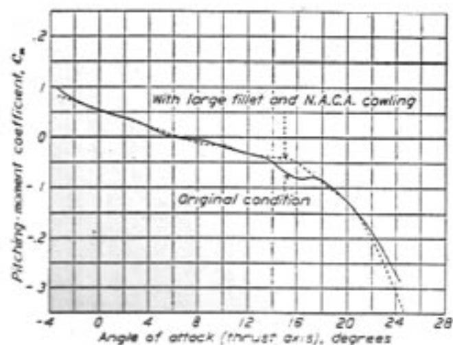
FIGURE 24.—Pitching moments of McDonnell airplane with power on. Corrected for tunnel effects. Stabilizer 0.5^\circ to thrust axis. Elevator 0^\circ to stabilizer.
