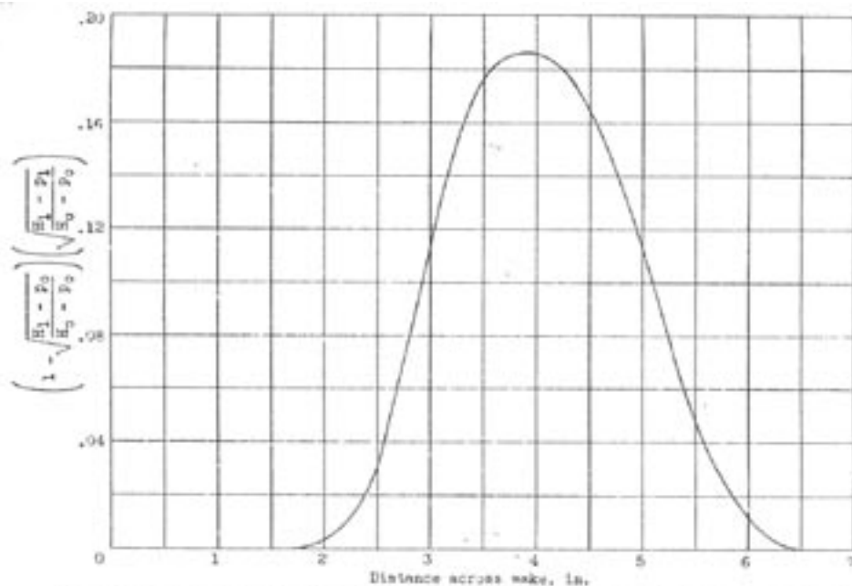
Figure 11.- Wake-survey curve for Lockheed 12-A wing with rubber de-icer and simulated ice on leading edge. Air speed, 175 miles per hour; chord at survey head, 81.3 inches.
