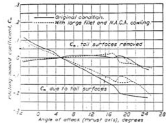
FIGURE 23.—Pitching moments due to tail of McDonnell airplane. Corrected for tunnel effects. Power off. Stabilizer 0.6° to thrust axis. Elevator 0° to stabilizer.
