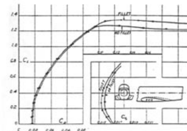
FIG. 15 LEFT AND DRAG POLAR CURVES FOR THE CASE OF A FILLET WING COMBINATION IN WHICH THE FUSELAGE IS STRAIGHT
