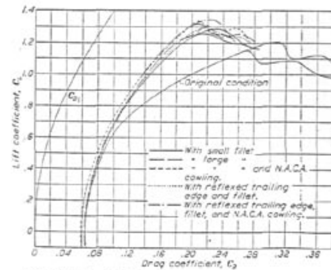
FIGURE 12.—Polars for 36-foot winged airplane with various fillets. Corrected for tunnel effects. Power off.
