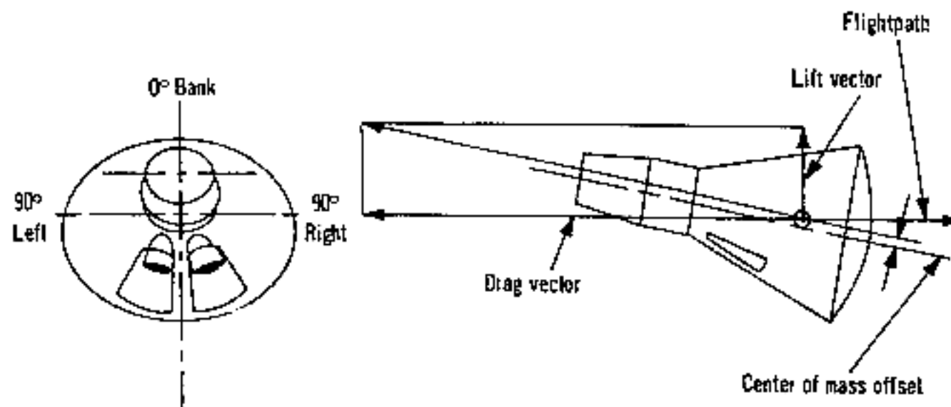
Figure 3.—Gemini vehicle trim condition.
