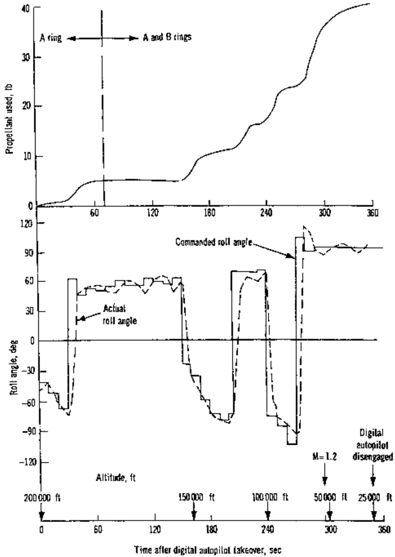
Figure 11.—Apollo 7 entry data.
