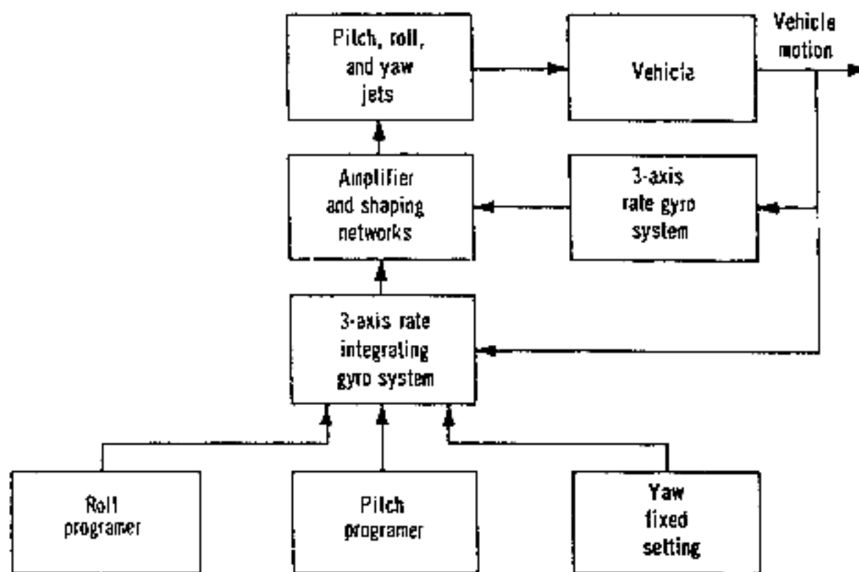
Figure 16.--ASSET guidance and control system.
