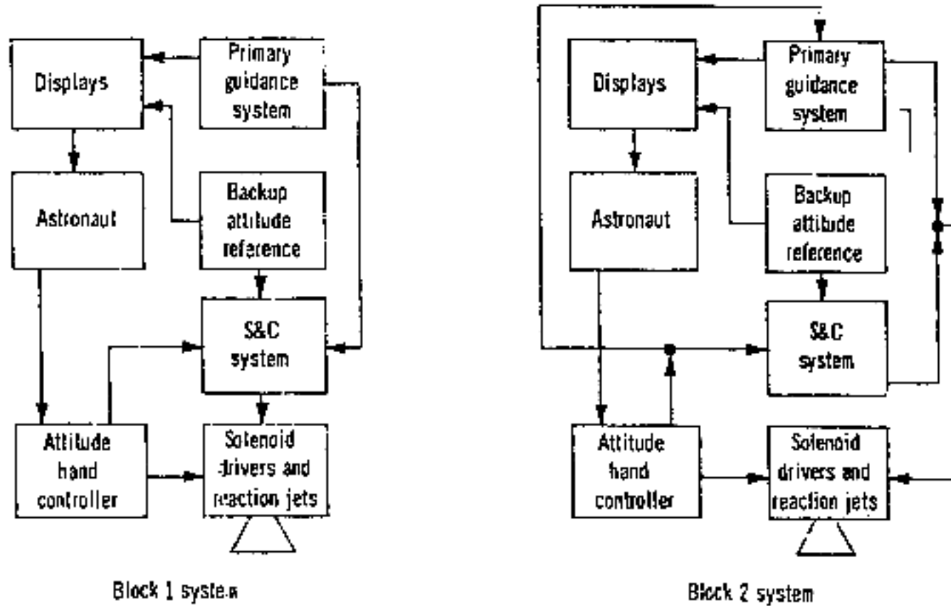
Figure 7.—Apollo G&C system designs.
