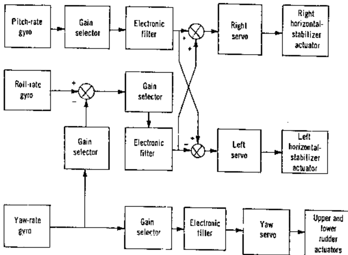
Figure 13.—Functional diagram of the stability augmentation system (SAS).
