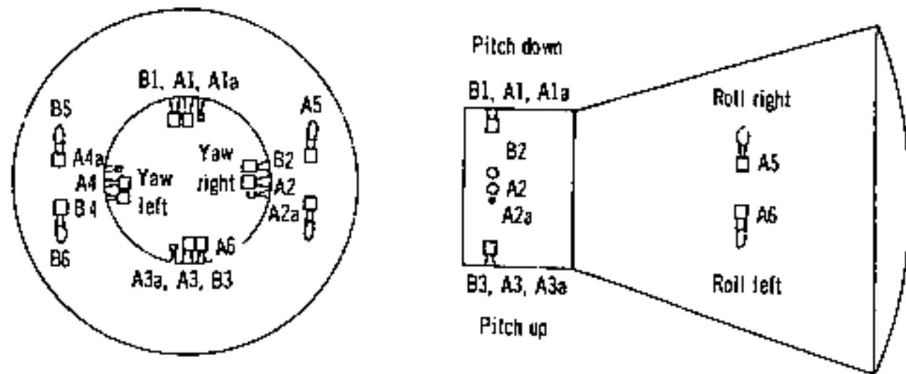
Figure 2.—Mercury entry-control jet configuration.
