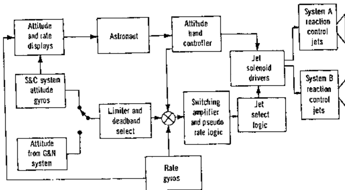
Figure 8.—Apollo entry-control functional diagram.
