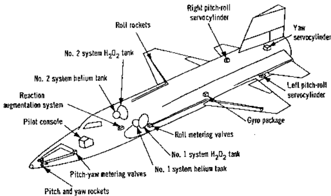
Figure 12.—Location of control-system components in X-15.
