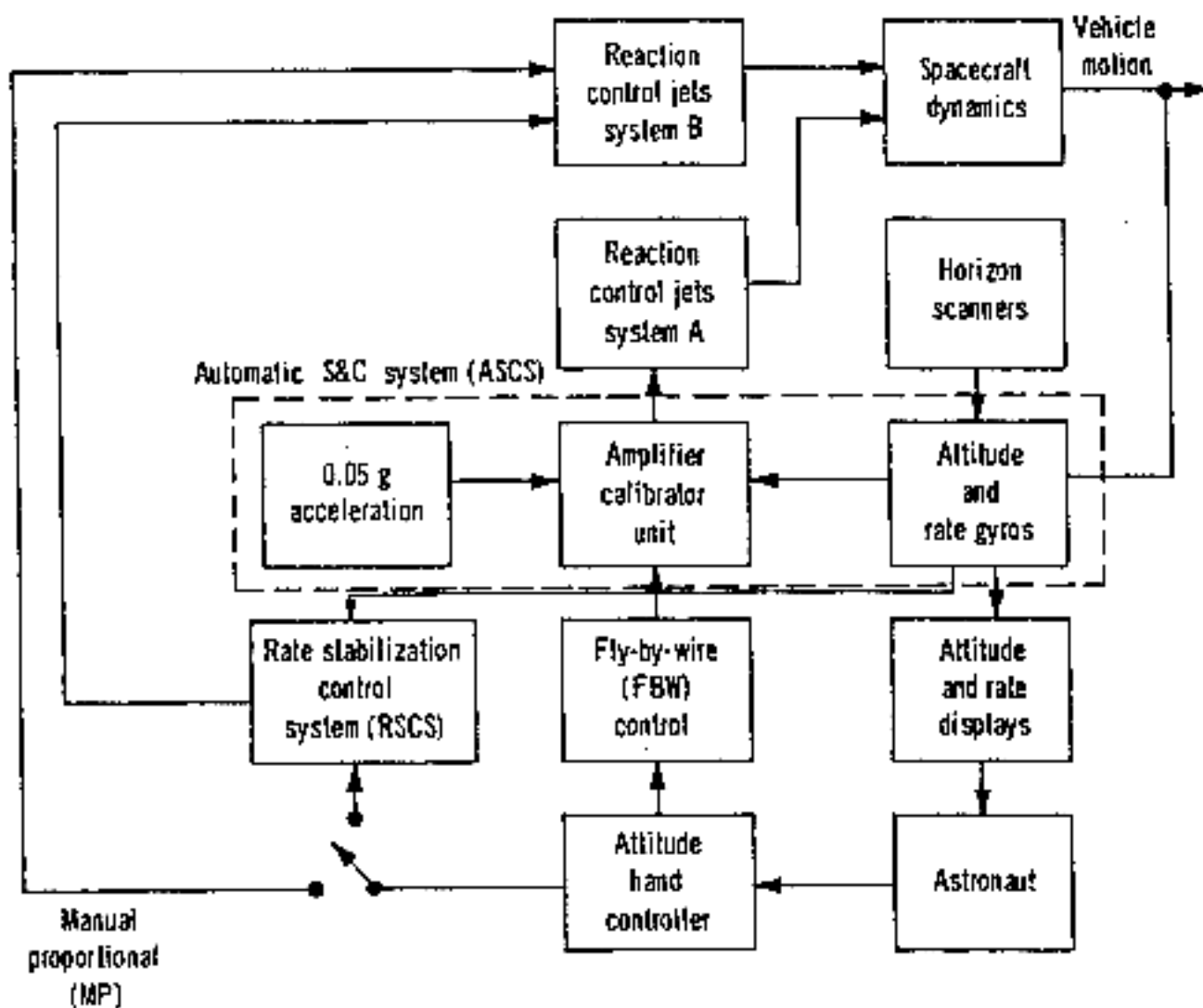
Figure 1.—Mercury control-system functional diagram.
