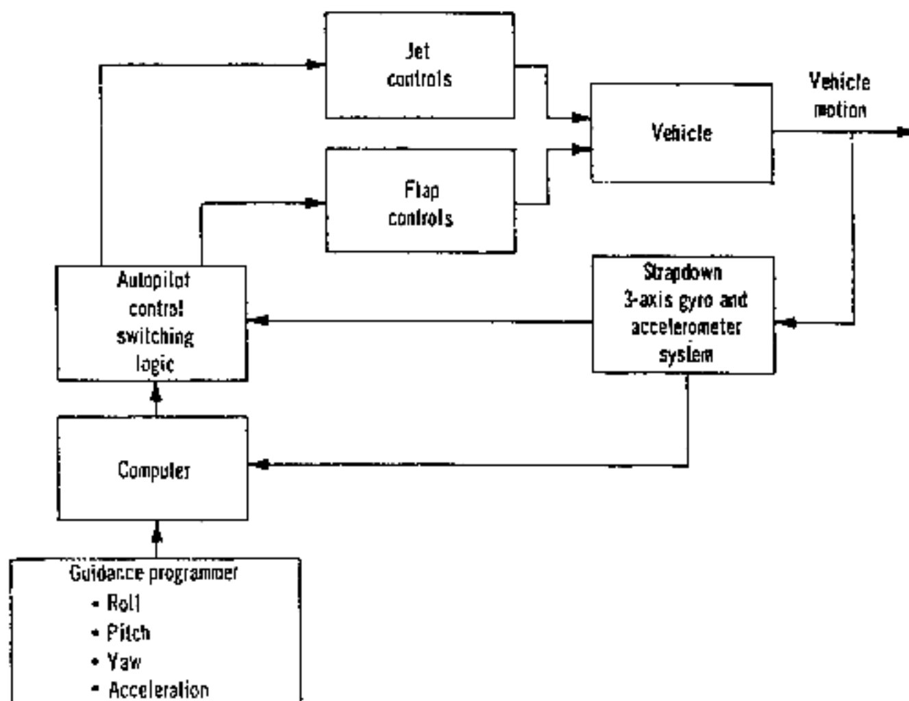
Figure 17.—PRIME entry G&C system.
