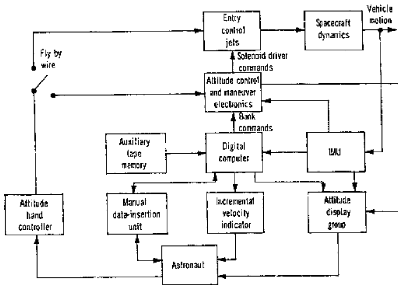
Figure 4.—Gemini entry G&C system.
