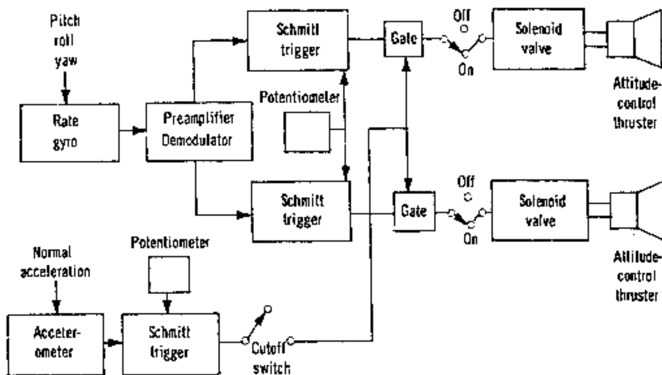
Figure 15.—Typical axis of X-15 reaction augmentation system.
