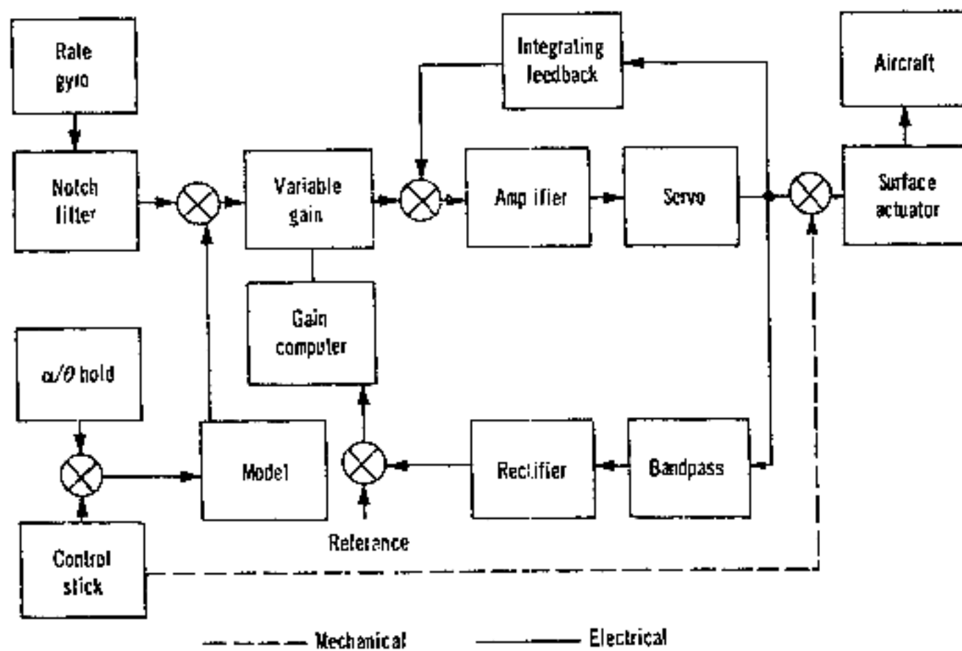
Figure 14.—MH-96 adaptive control-system pitch mode.
