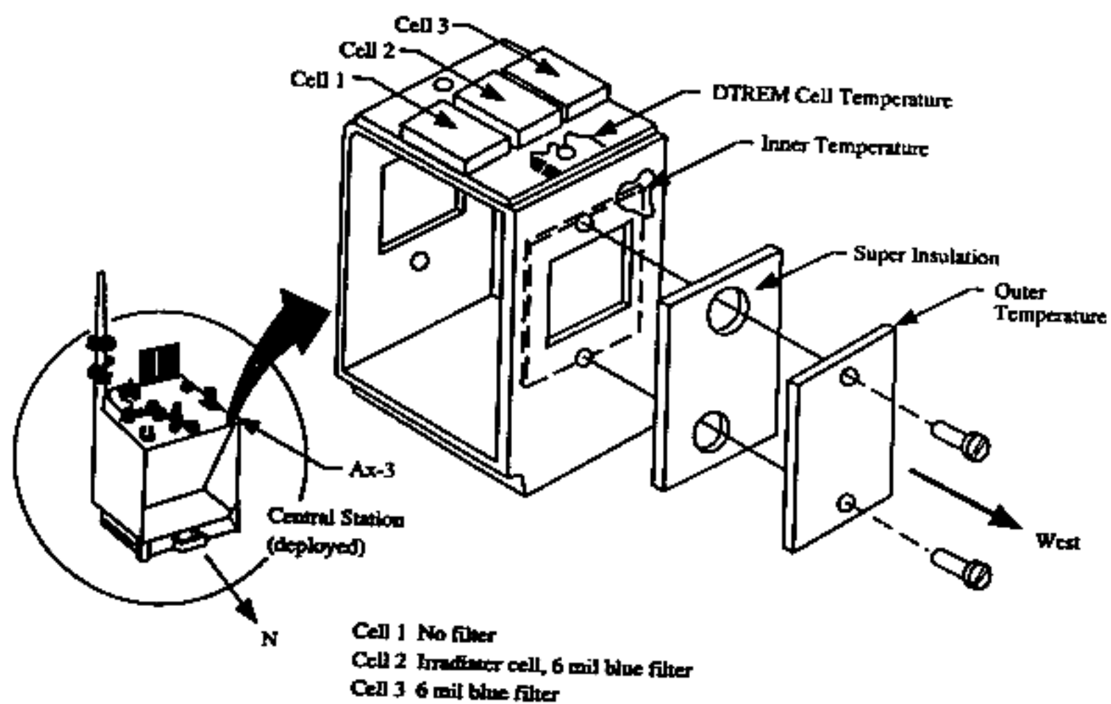
Figure 7. DTREM schematic.
