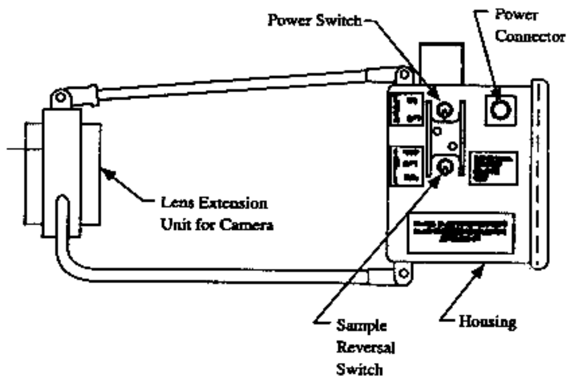
Figure 40: Electrophoresis demonstration - left side view.
