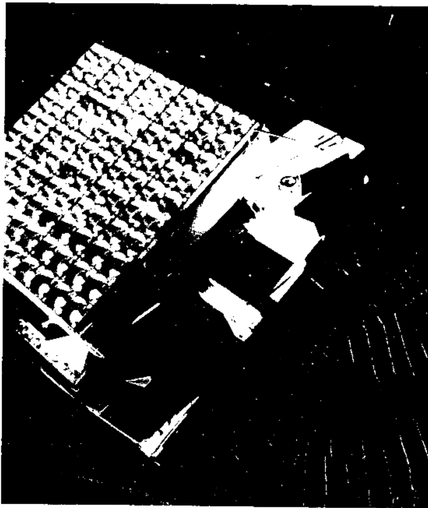
Figure 13: The LRRR as deployed at the Apollo 14 site. Note the bubble level and the shadow graph for orientation. These were set for the landing site location prior to launch (AS-14-67-9385). See also figure 8 for a method of carrying the LRRR.
