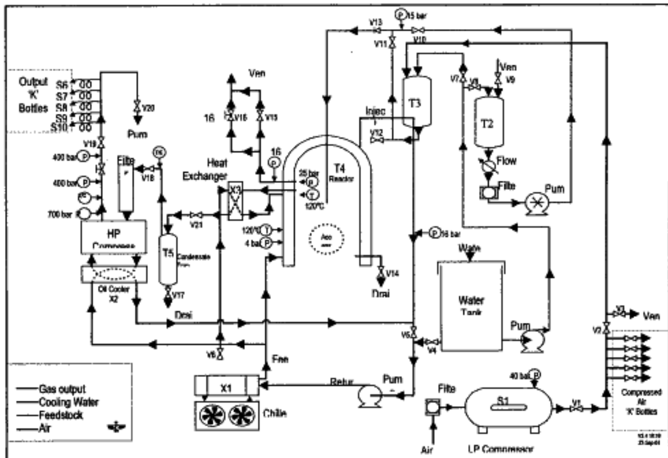
Figure 9. Process flow diagram of trailer process.
