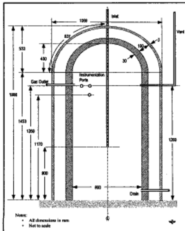
Figure 10. Diagram of reactor.
