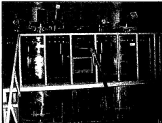
Figure 4. Two 1,000-liter, stirred, jacketed vessels suitable for use as fermentors for the growth of bacterial BW agents.
